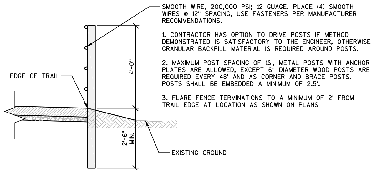
FENCE INSTALLATION DETAIL
