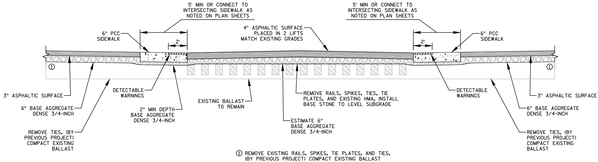
TYPICAL FINISHED SECTION RECONSTRUCTION AT STREET CROSSINGS: JOHN QUINCY ADAMS STREET JACKSON STREET/FRANKLIN STREET WASHINGTON AVENUE WASHINGTON STREET HEMLOCK STREET
