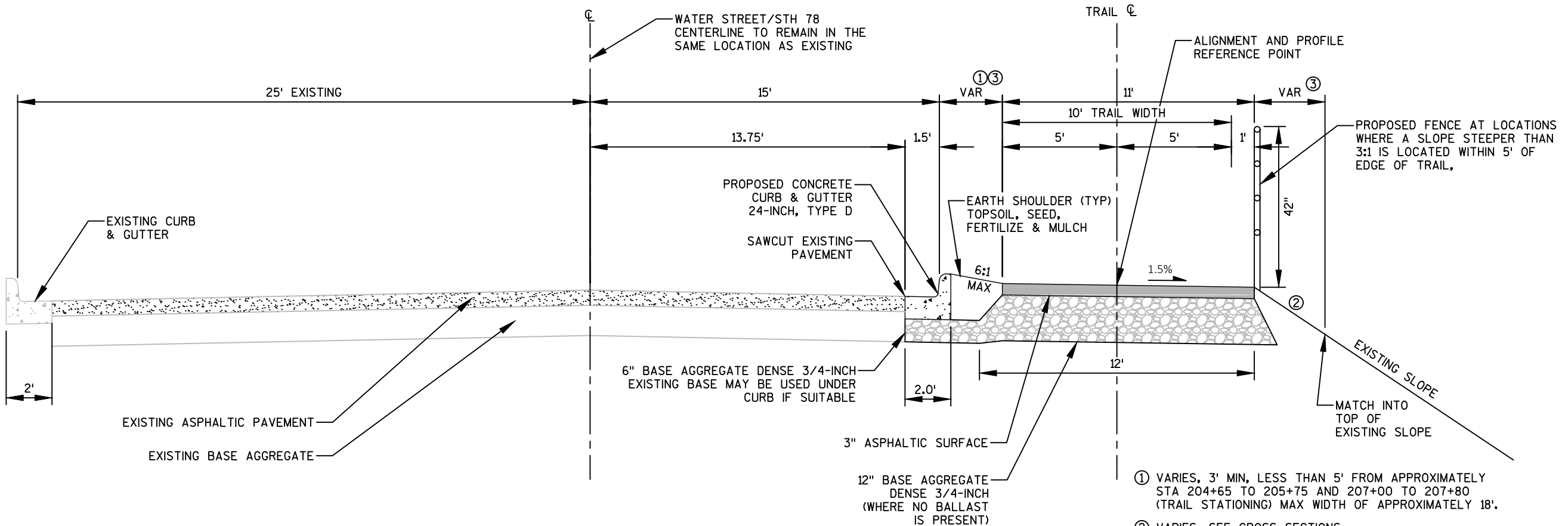
TYPICAL FINISHED SECTION WATER STREET/STH 78 & PARALLEL GREAT SAUK TRAIL STA 202+30 TO STA 207+50
