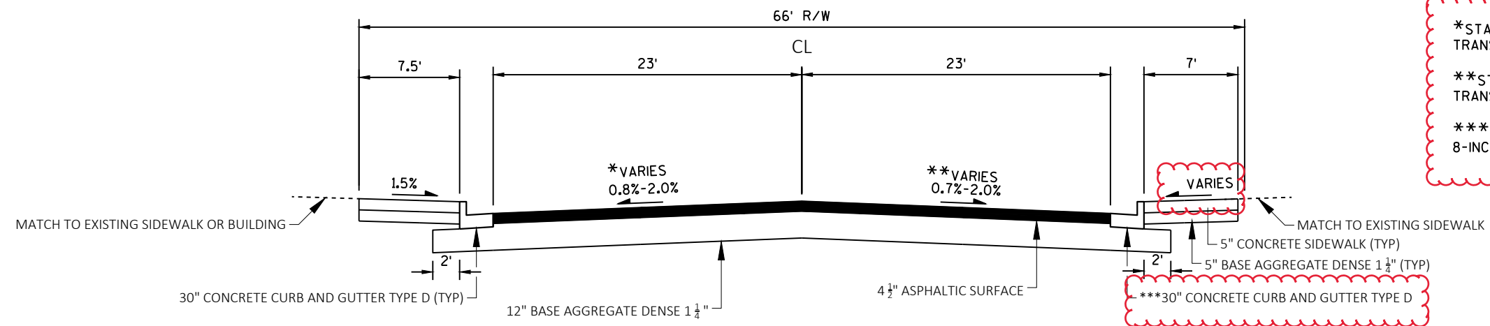
TYPICAL FINISHED SECTION NORTH BRISTOL STREET 40'NB'+51.28 TO 42'NB'+30.56
