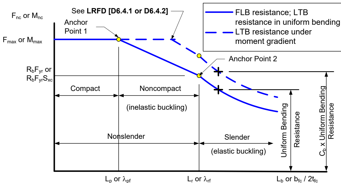
Figure 24.1-5 Form of the Compression-Flange Resistance Equations in AASHTO LRFD
