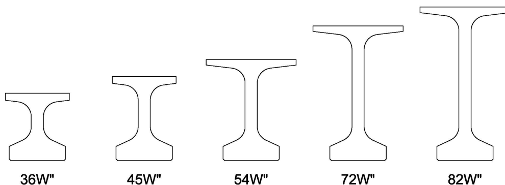
WisDOT Wide Flange Girder Shapes
