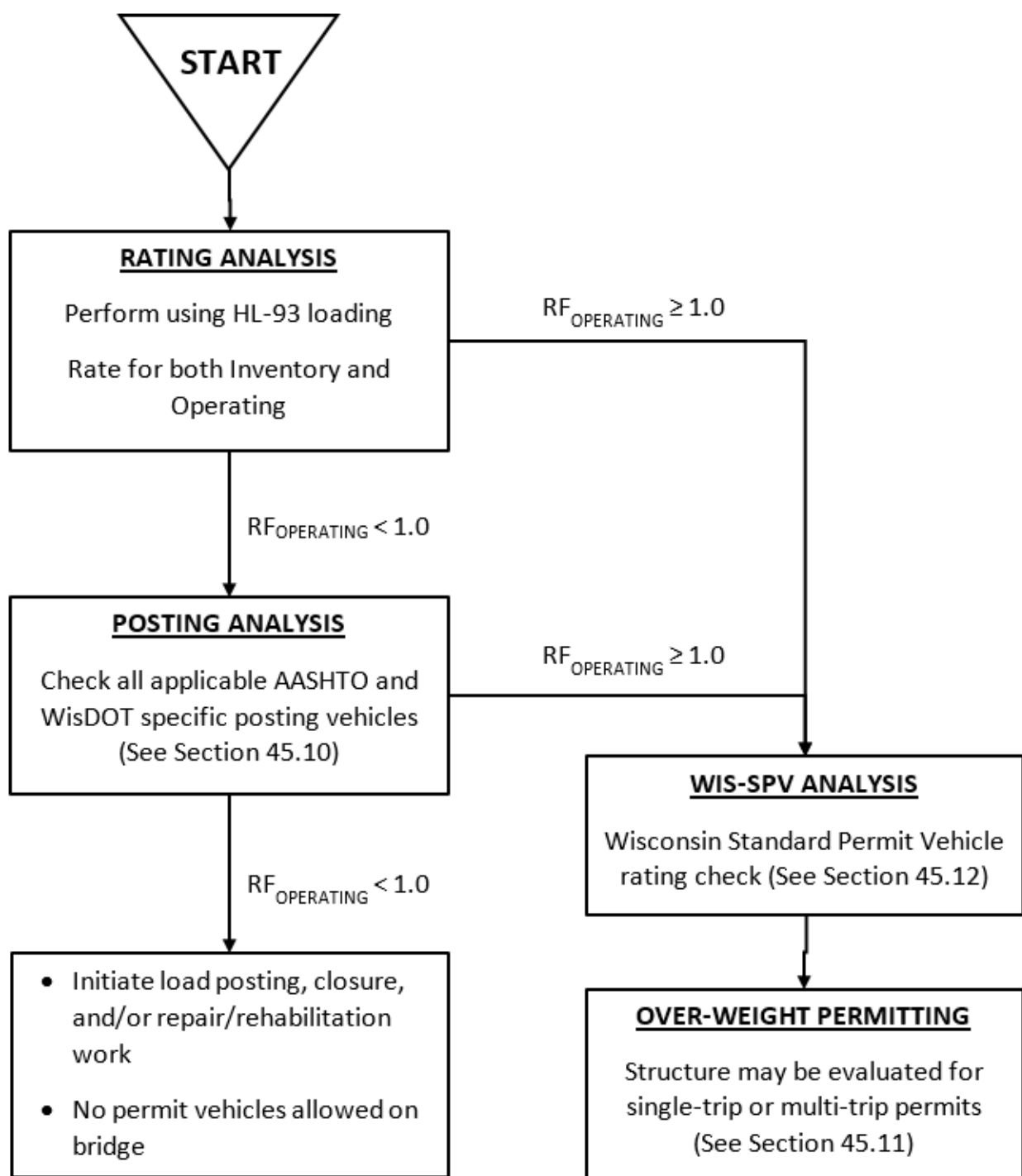
Figure 45.3-1 Load and Resistance Factor Rating Flow Chart
