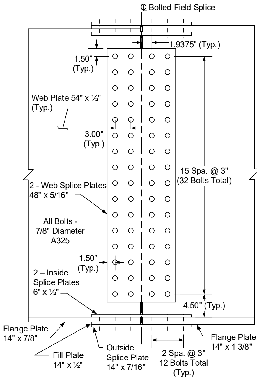
Figure 24.8-7 Sample Schematic of Final Splice Configuration
