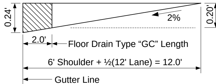
Figure 29.3-1 Cross Section of Flow
