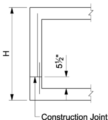
Figure 36.6-4 Layout of Exterior Wall Steel
