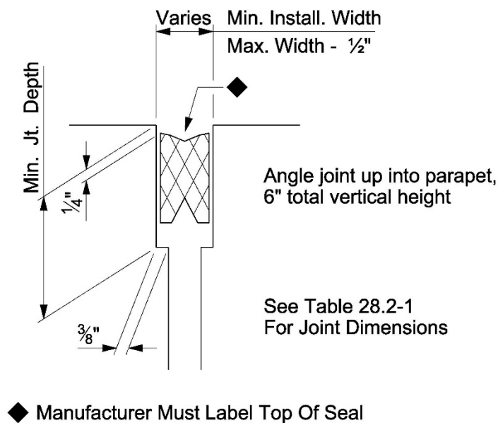
Figure 28.2-1 . Joint Design
