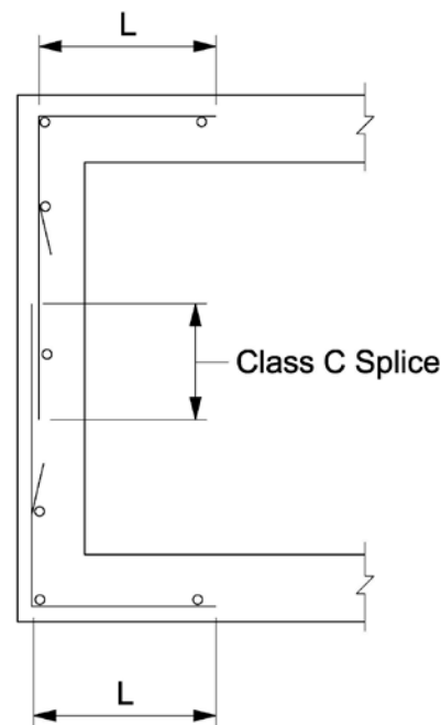
Figure 36.6-1 Layout of Corner Steel
