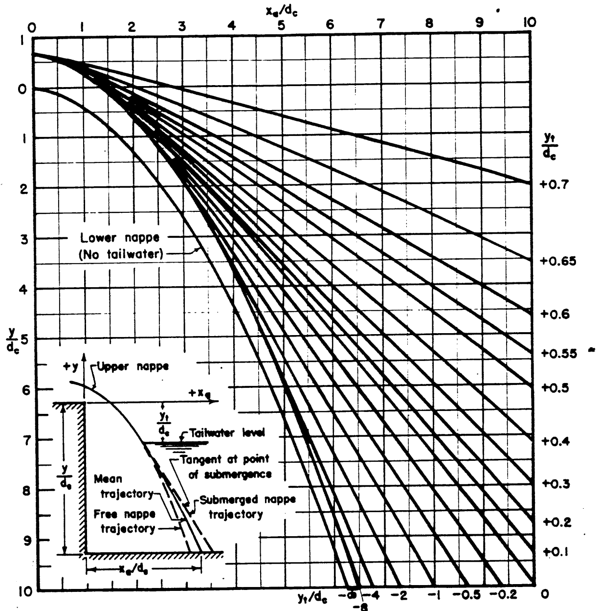
Figure 8.4-9 Design Chart for Determination of "X a "
