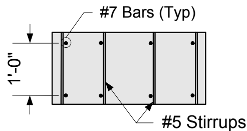
Figure E13-1.8-9 Crack Control Reinforcement - Option 1
