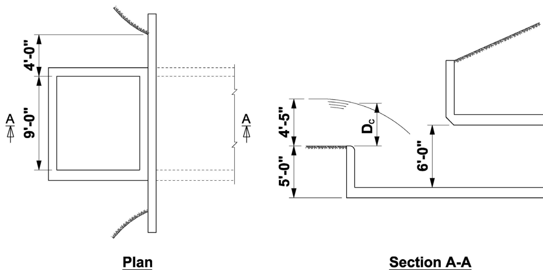
Figure 8.4-8 Drop Inlet Example
