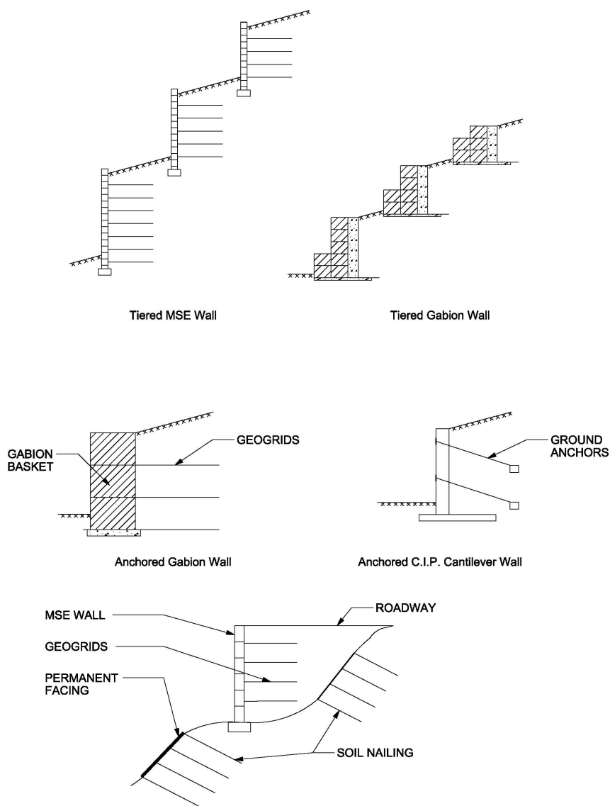
Figure 14.2-3 Tiered & Hybrid Wall Systems
