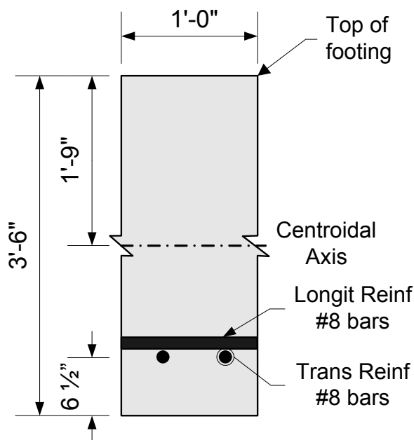
Figure E13-1.11-1 Footing Cracking Moment Dimensions
