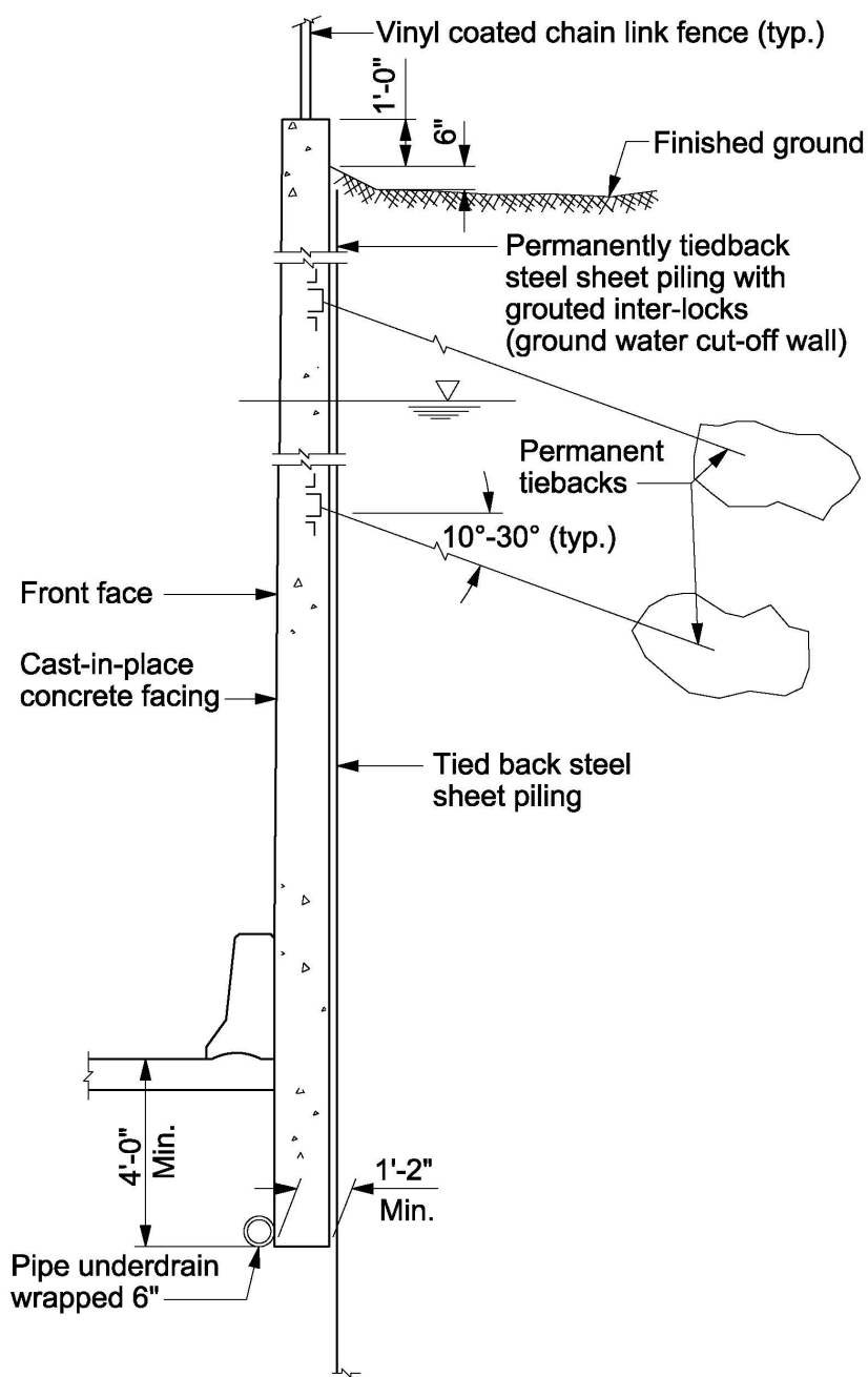
Typical Section - Tiedback Retaining Wall
