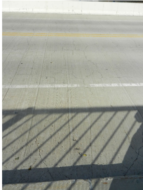
Bridge B-40-376 Deck Cracks
