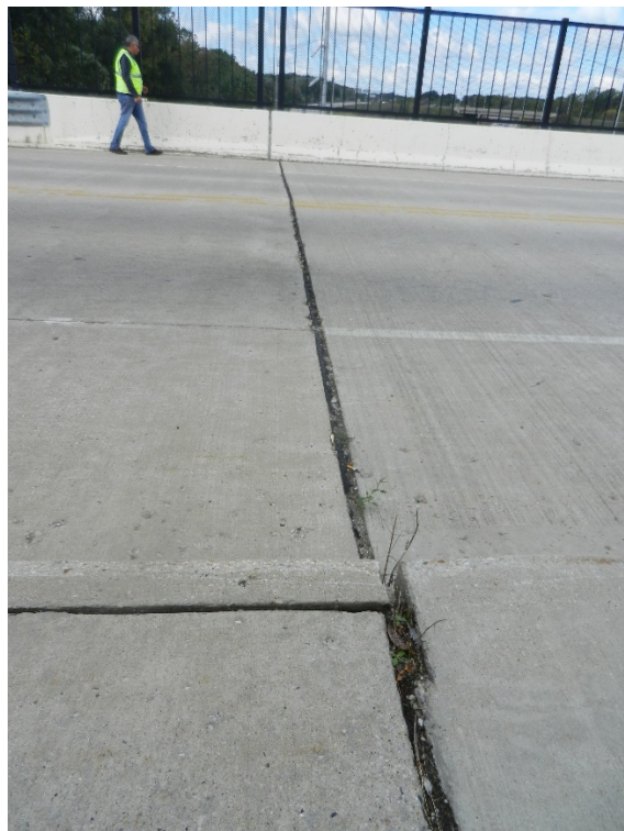
Bridge B-40-376 South Approach Joint
