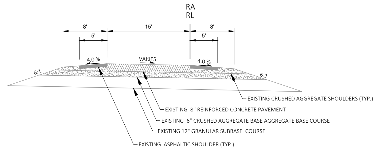
EXISTING RAMP TYPICAL SECTION WISDOT REST AREA NO. 33 (RA LINE)
