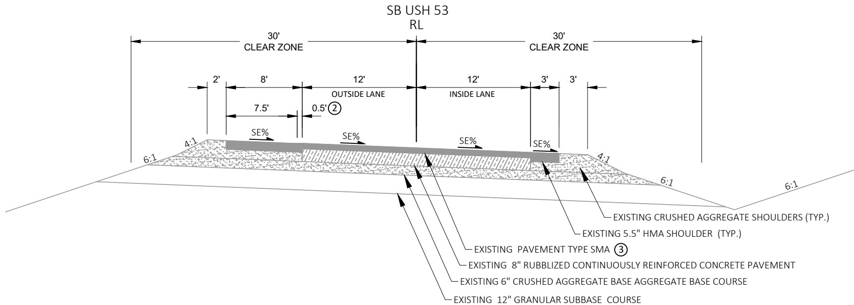
EXISTING TYPICAL SUPERELEVATION SECTION (SEE PLAN SHEET FOR LOCATIONS)
