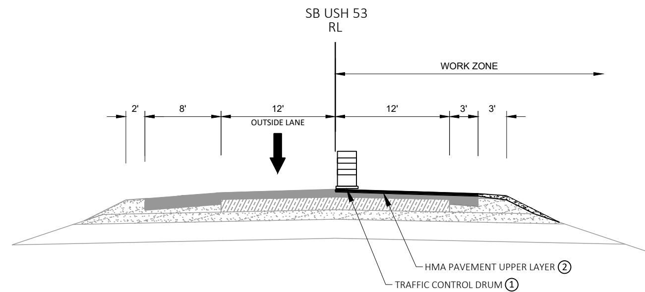
CONSTRUCTION STAGE 4 TYPICAL SECTION (LOOKING NORTH)
