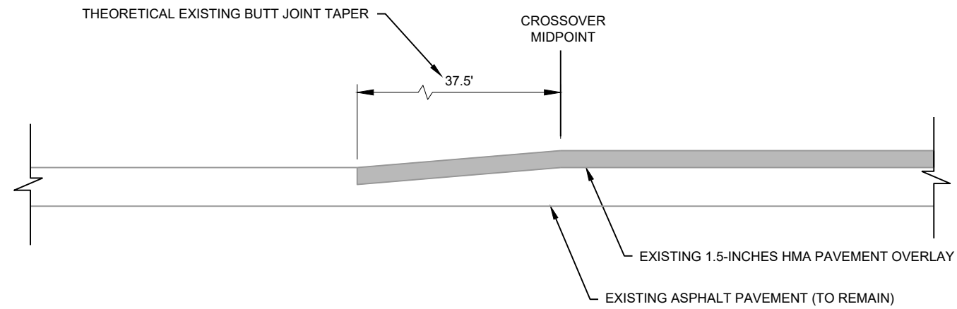
SECTION A-A - EXISTING CONDITION
