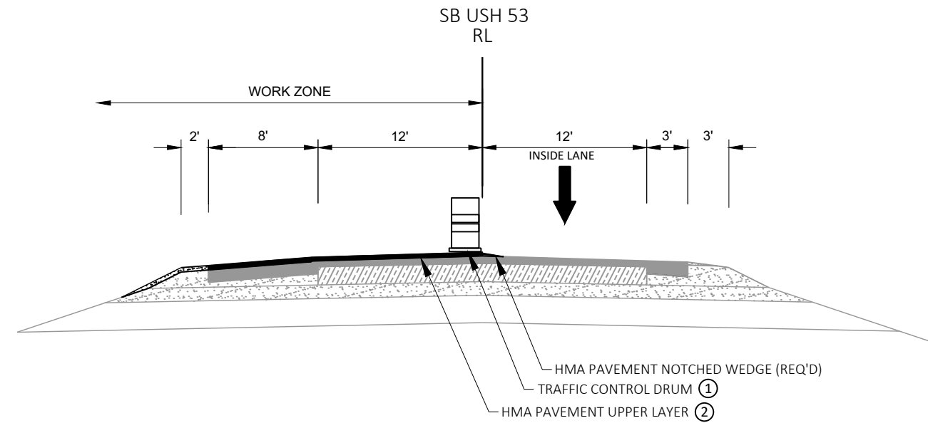
CONSTRUCTION STAGE 3 TYPICAL SECTION (LOOKING NORTH)
