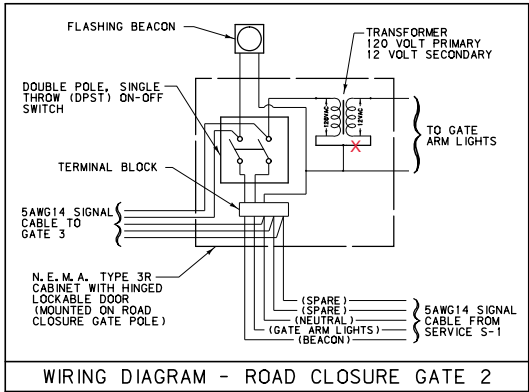
WIRING DIAGRAM - ROAD CLOSURE GATE 2
