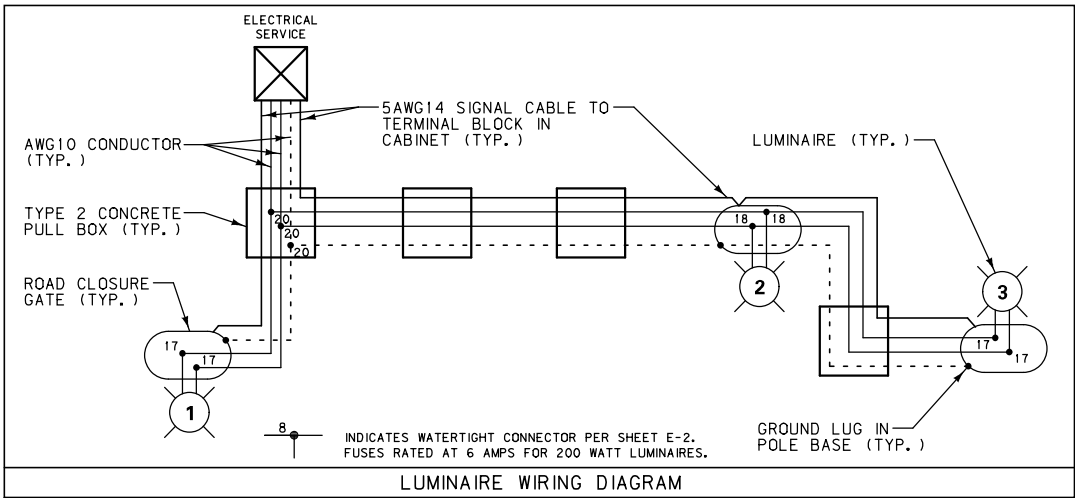
LUMINAIRE WIRING DIAGRAM
