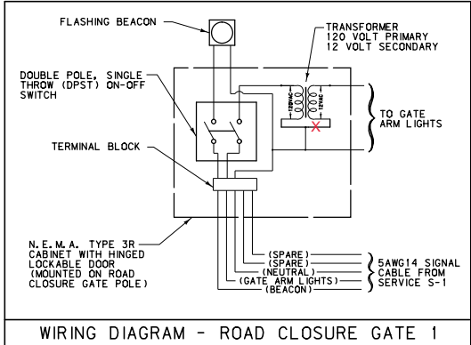
WIRING DIAGRAM - ROAD CLOSURE GATE 1
