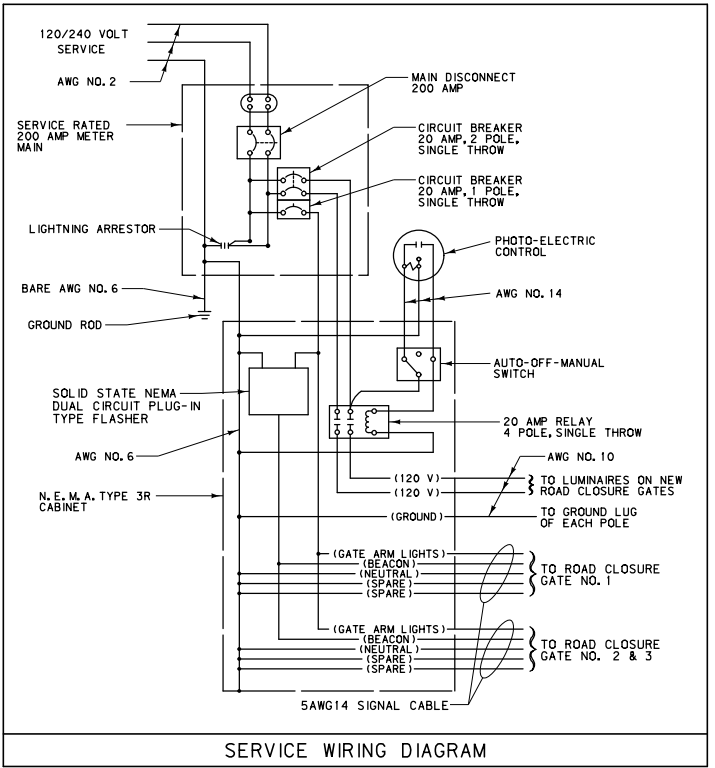
SERVICE WIRING DIAGRAM
