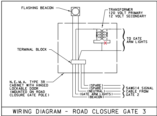
WIRING DIAGRAM - ROAD CLOSURE GATE 3
