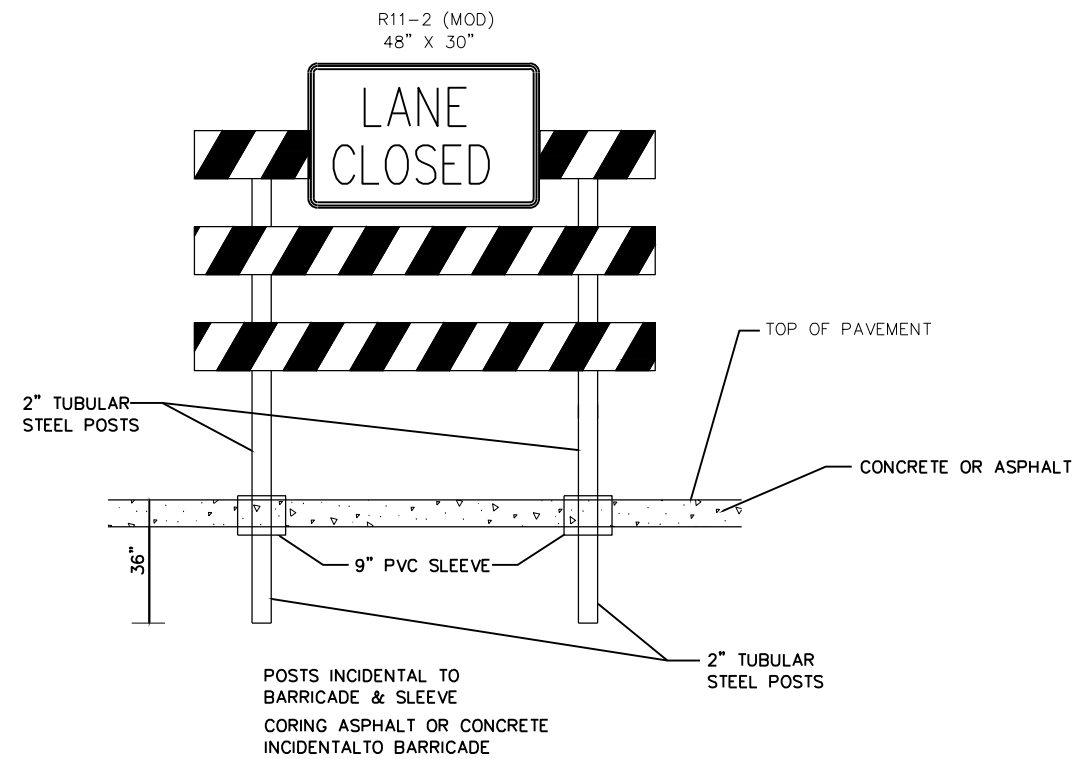
TRAFFIC CONTROL BARRICADE PERMANENT TYPE III ANCHORING DETAIL WITH SLEEVES
