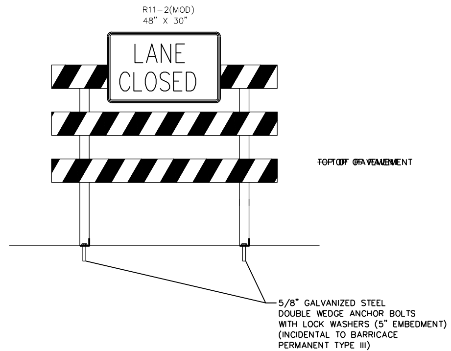
TRAFFIC CONTROL BARRICADE PERMANENT TYPE III ANCHORING DETAIL WITH CLIPS
