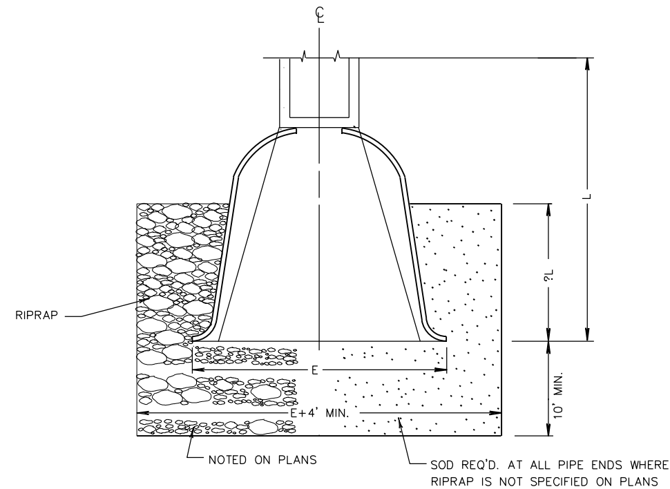
SOD OR RIPRAP AT PIPE END (SEE PLAN)
