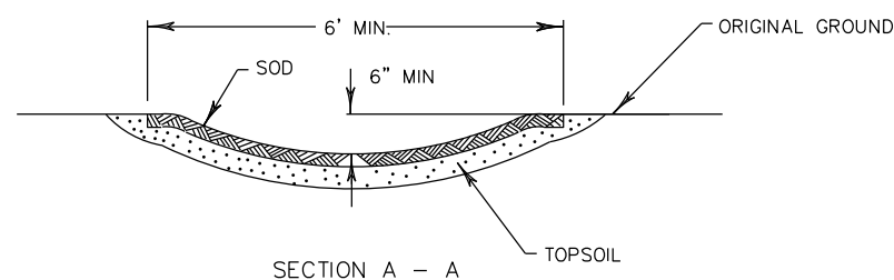
SOD DETAIL AT CURB ENDS
