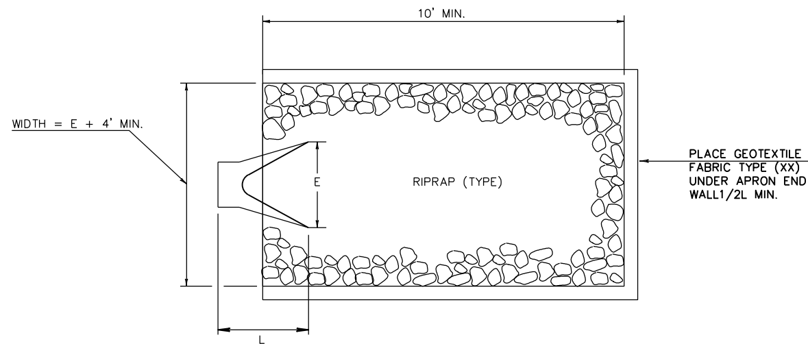
TYPICAL PLACEMENT OF RIPRAP AT CULVERT ENDS
