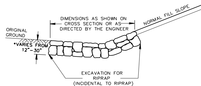
DETAIL FOR RIPRAP IN DITCHES
