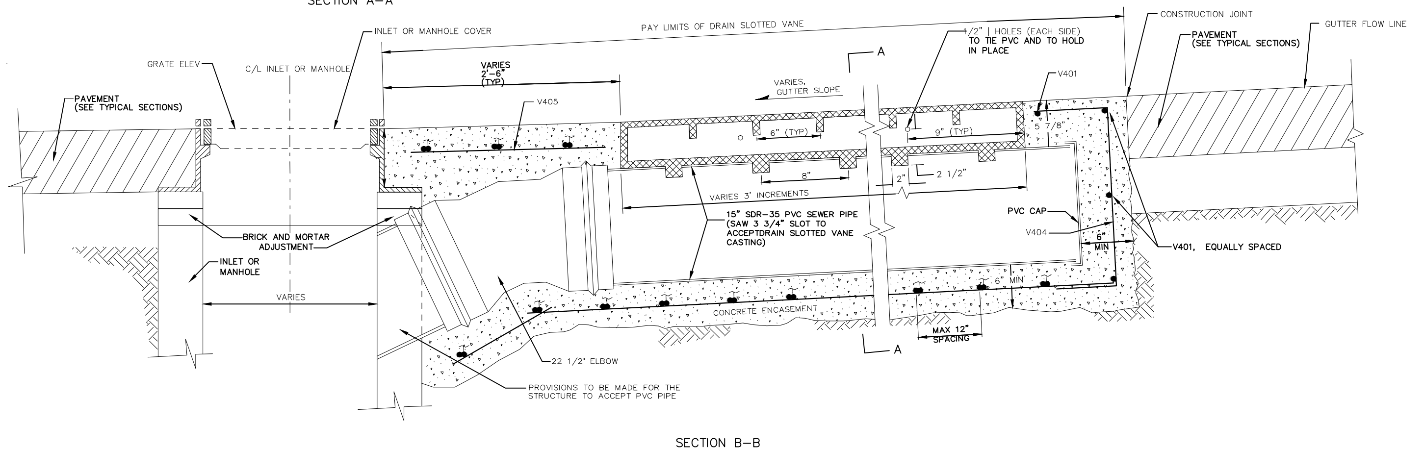
DRAIN SLOTTED VANE LONGITUDINAL AND DRAIN SLOTTED VANE LONGITUDINAL TEMPORARY
