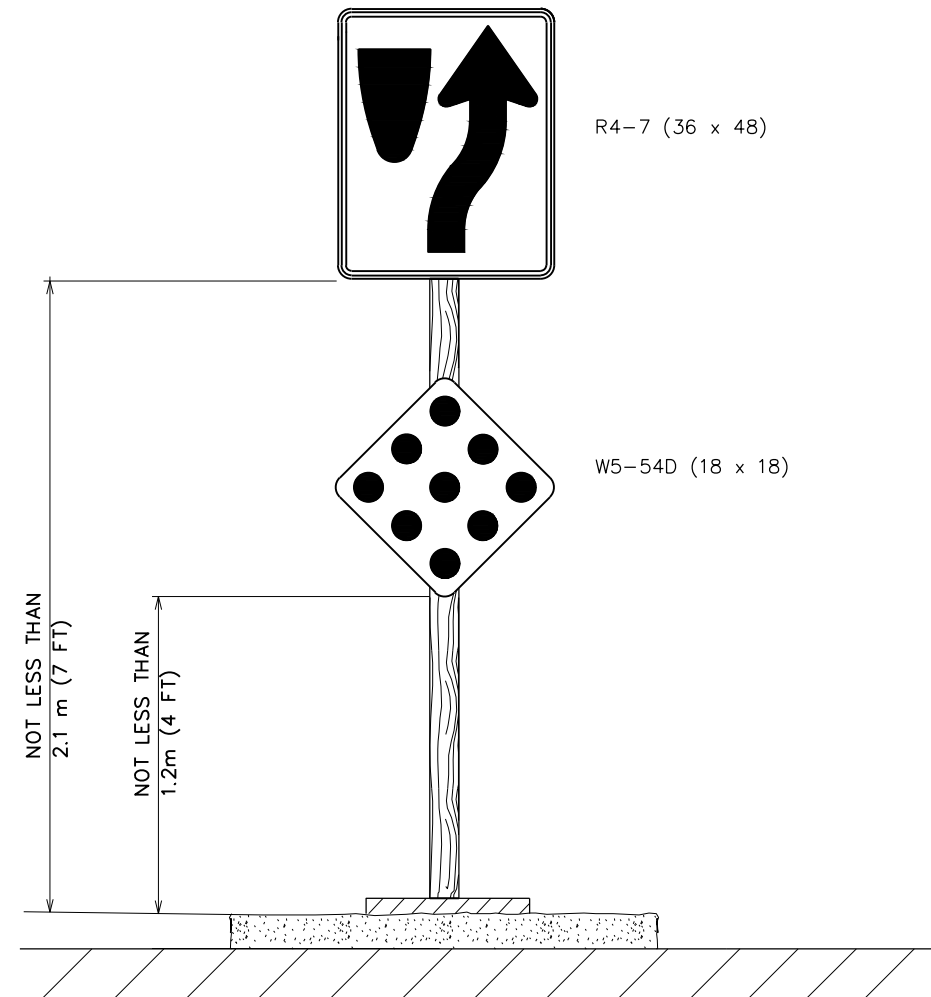
TYPICAL INSTALLATION FOR TRANSITION TO DIV. HIGHWAY OR OTHER SPECIAL NEEDS AREAS
