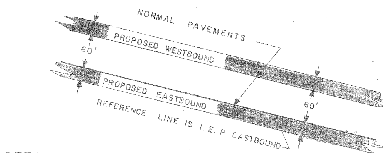
DETAIL OF NORMAL ROADWAY IN RELOCATION SCALE 1"=100'
