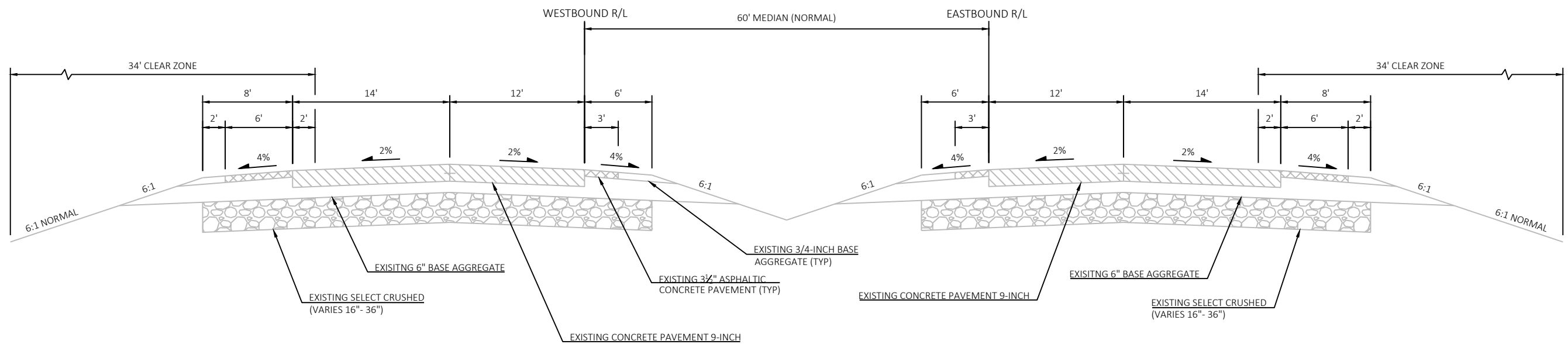
TYPICAL EXISTING CROSS SECTION FOR STH 23 STA 399+70 TO STA 425+89 STA 461+36.07 TO STA 511+32
