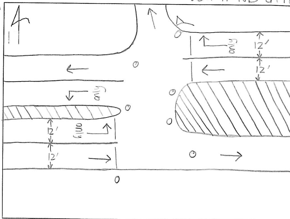
Diagram of Intersection USH 41 NB on ramp
