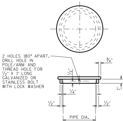
POST/END CAP DETAIL
