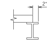
CATWALK TERMINATION DETAIL
