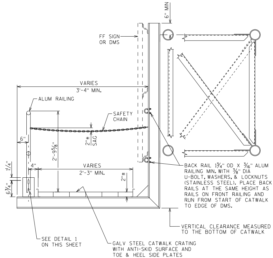
SECTION THRU WALKWAY
