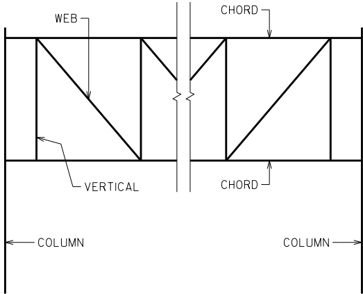
TWO CHORD TRUSS ORIENTATION
