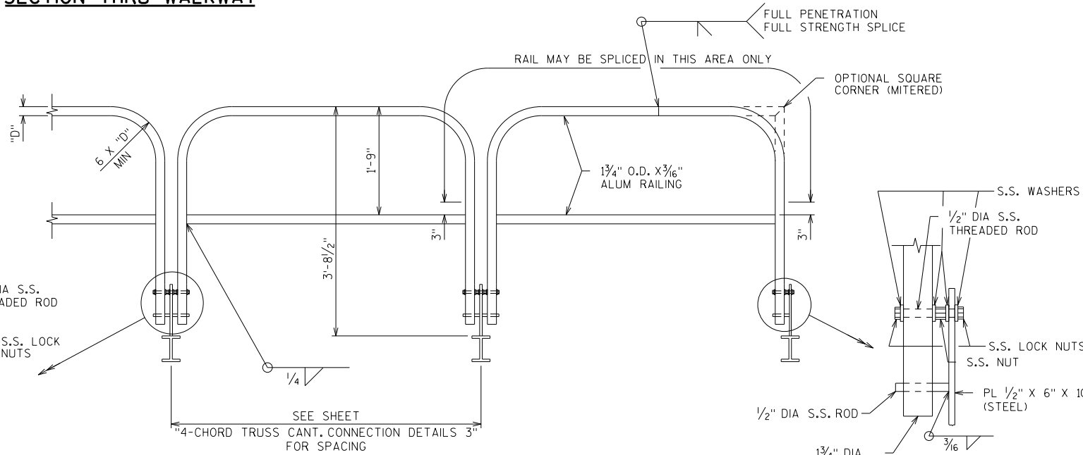
TYPICAL FRONT RAILING DETAILS
