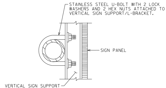
U-BOLT DETAIL
