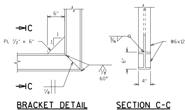
CATWALK TERMINATION DETAIL
