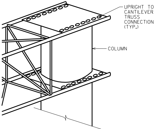
CANTIEVER SIGN BRIDGE
