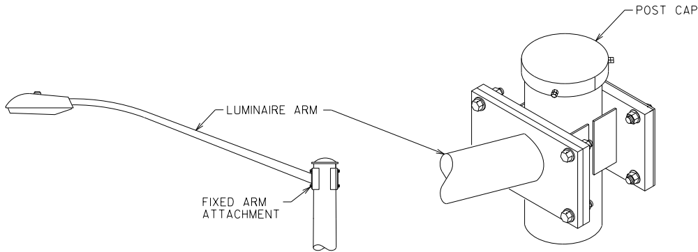
POST TO LUMINAIRE ARM CONNECTION WIRING TO RUN INSIDE LUMINAIRE ARM
