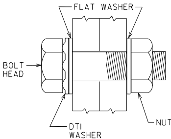
RECOMMENDED BOLT ASSEMBLY DETAIL
