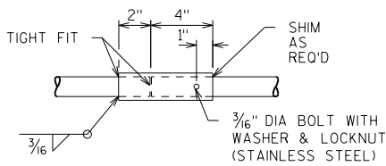
BACKRAIL SPLICE
