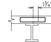
CATWALK SPLICE LOCATION DETAIL
