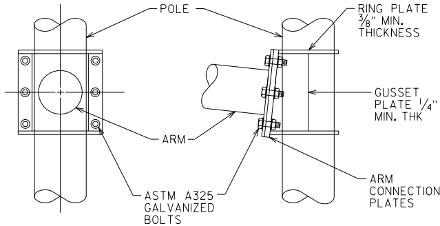
POST TO MAST ARM CONNECTION
