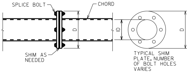
SPLICE CONNECTION BOLT DETAIL
