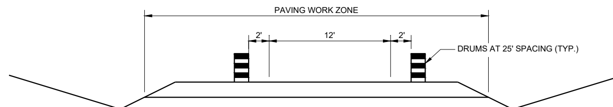
STAGE III - TRAFFIC ON BASE COURSE
