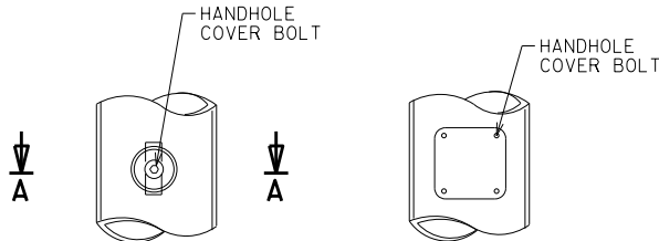
HANDHOLE DETAILS
