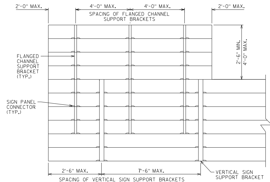
FLANGED CHANNEL SUPPORT/VERTICAL SIGN SUPPORT BRACKET DETAILS
