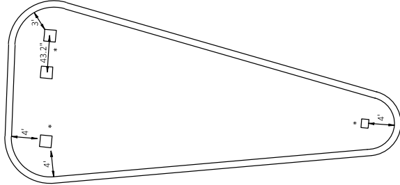
DETAIL OF OPENINGS IN ISLAND FOR SIGN PLACEMENT
