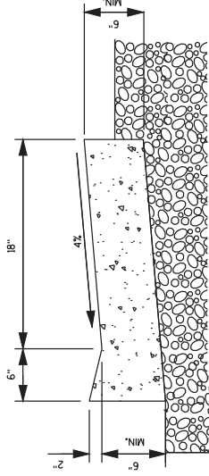
CRUSHED AGGREGATE BASE COURSE DRIVEWAY ENTRANCE CURB
