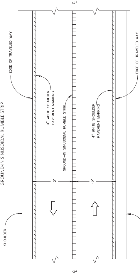
CENTER LINE SINUSOIDAL GROOVES ON TWO-WAY ROADWAYS ASPHALTIC CENTERLINE RUMBLE STRIPS, SINUSOIDAL, 2-LANE RURAL
