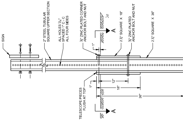
DETAIL OF TUBULAR STEEL SIGN POST
