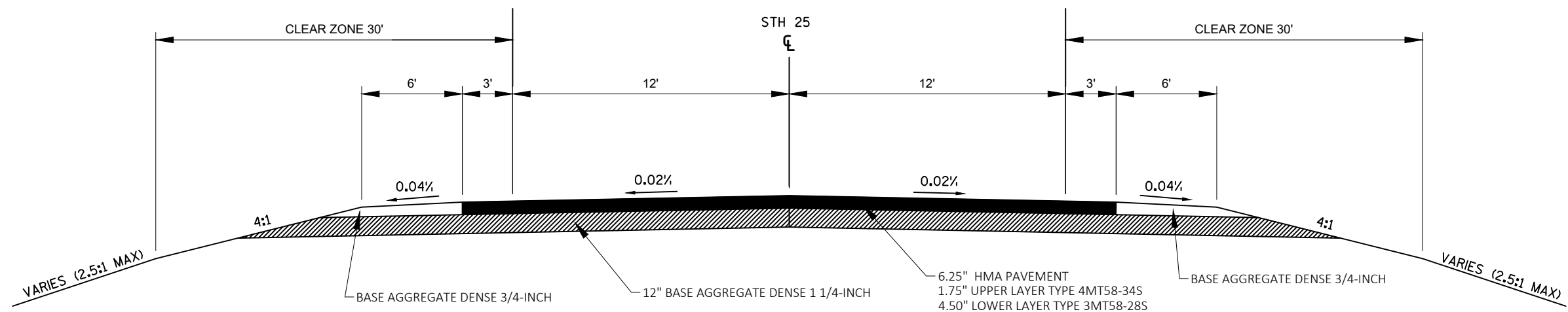
STH 25 PROPOSED TYPICAL SECTION 174+24.94-176+40.67
