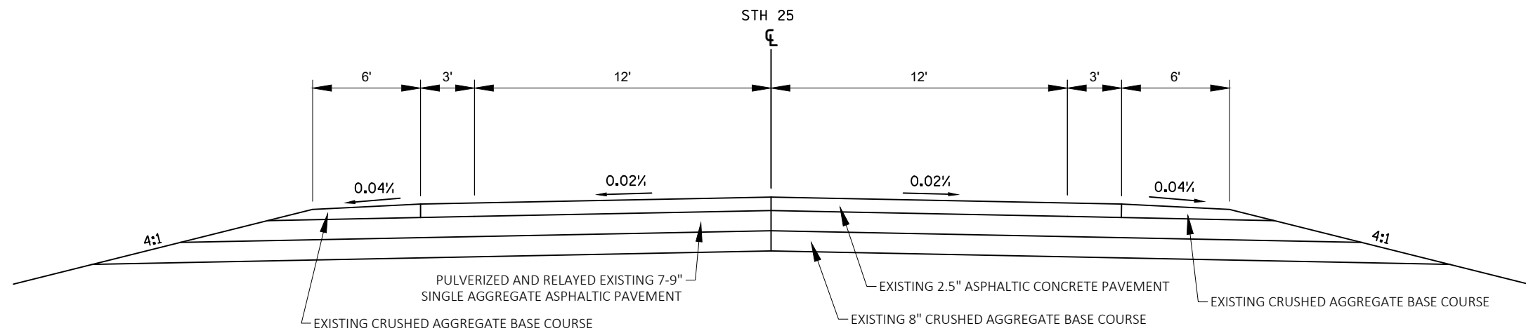
STH 25 EXISTING TYPICAL SECTION 174+24.94-176+40.67
