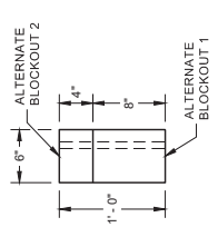
PLAN VIEW
