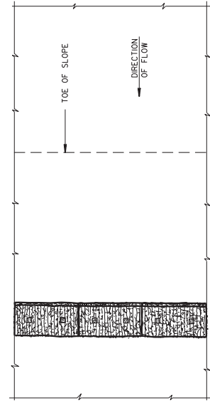
PLAN VIEW
