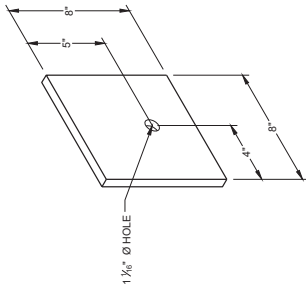
BEARING PLATE (E)
