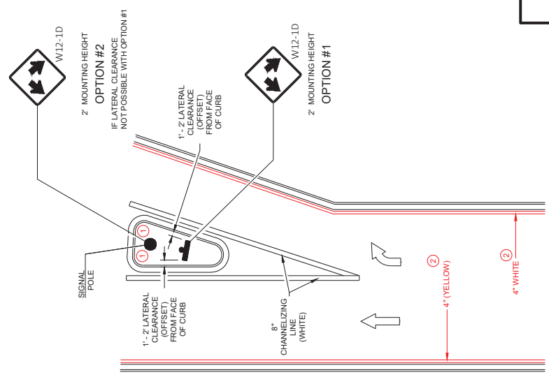
RIGHT TURN ISLAND
