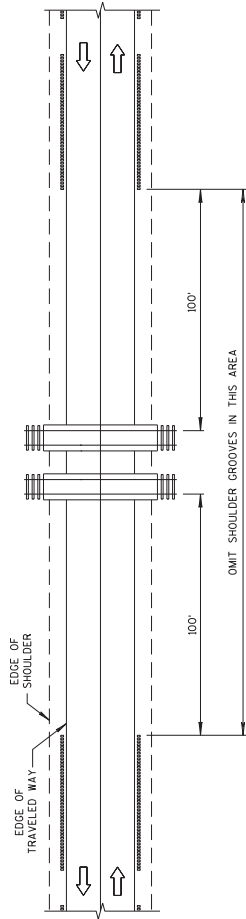
SHOULDER GROOVES AT RAILROADS
