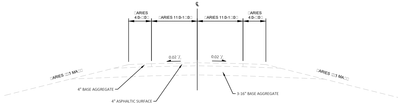
TYPICAL EXISTING SECTION CTH Q
