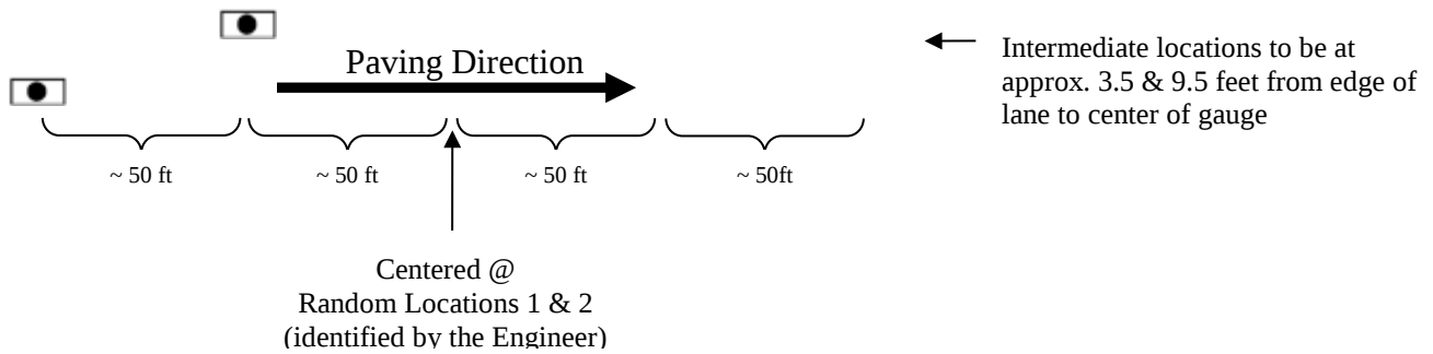
Figure 1: Nuclear/Core Correlation Location Layout
