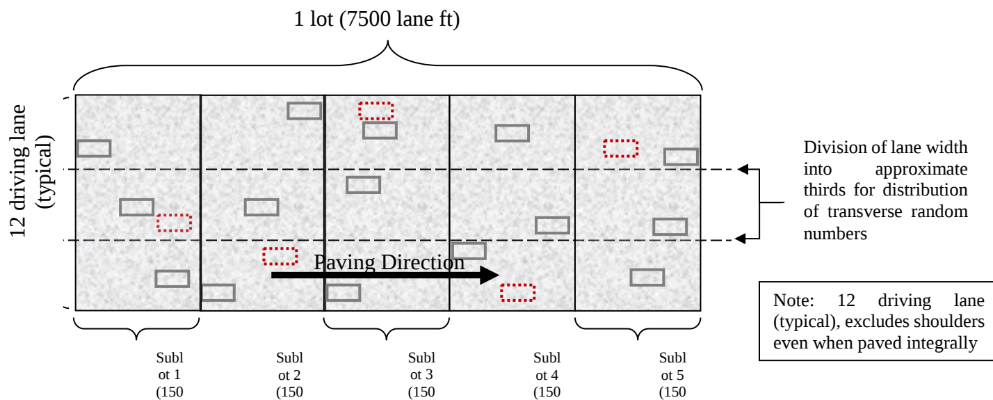
Figure 5: Locations of main lane HMA density testing (QC=solid lines, QV=dashed)
