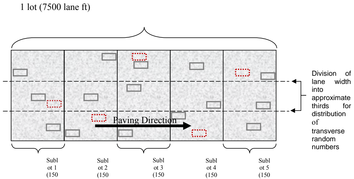
Figure 3: Locations of main lane HMA density testing (QC=solid lines, QV=dashed)
