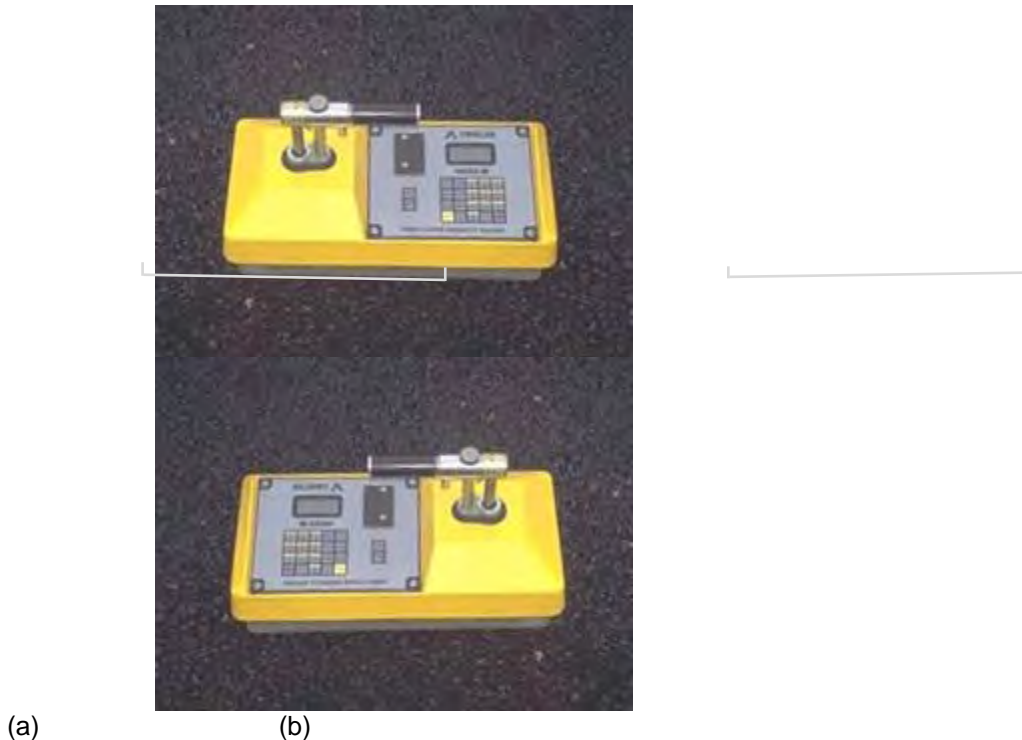
Figure 2: Nuclear gauge orientation for (a) 1 st one-minute reading and (b) 2 nd one-minute reading
