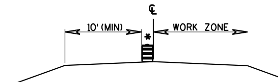
TRAFFIC LAYOUT - WORKING HOURS
