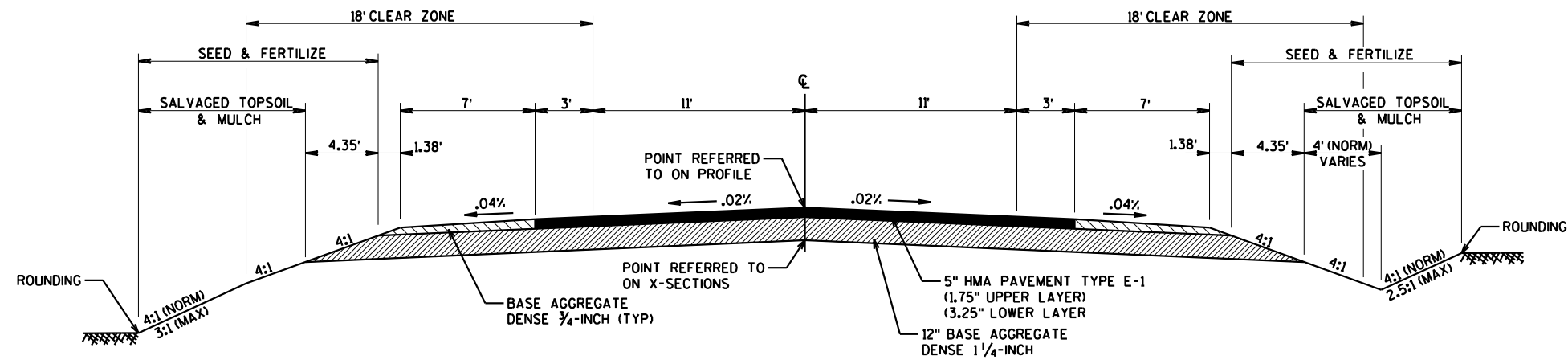
FINISHED TYPICAL SECTION CTH A (RECONSTRUCT) STA 102+55.57 - STA 107+00.00
