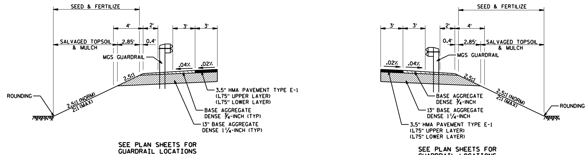
FINISHED TYPICAL SECTION CTH A (RECONDITION) STA 107+00.00 - STA 371+00.00
