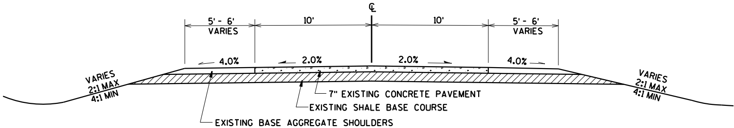
EXISTING TYPICAL SECTION CTH A
