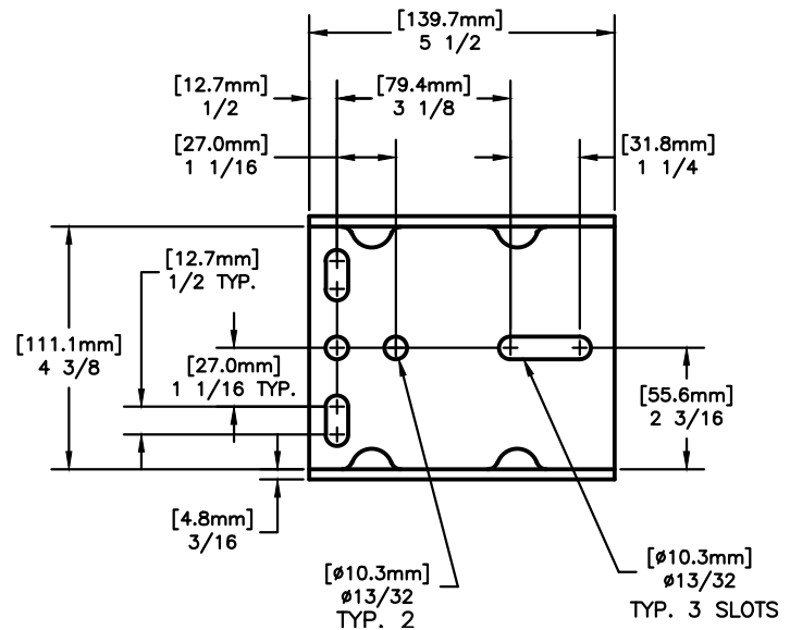
BASE HOLE PATTERN
