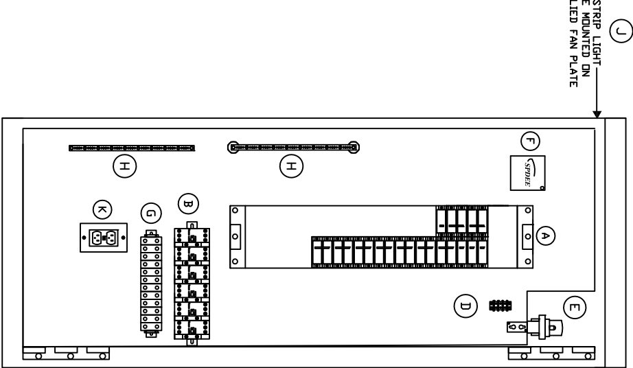
BACK PANEL VIEW DEAD FRONT REMOVED
