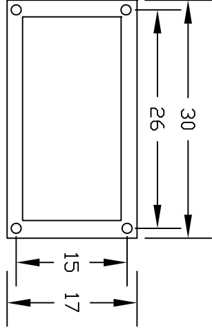
MOUNTING DETAIL
