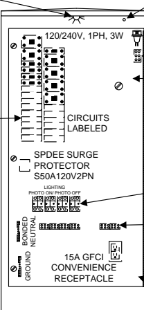
INTERIOR COMPONENTS
