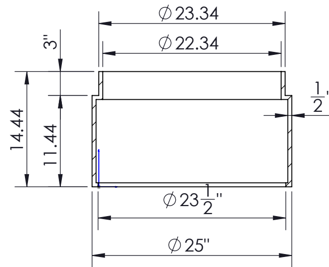
D - 12" EXTENSION (2412HD5)
