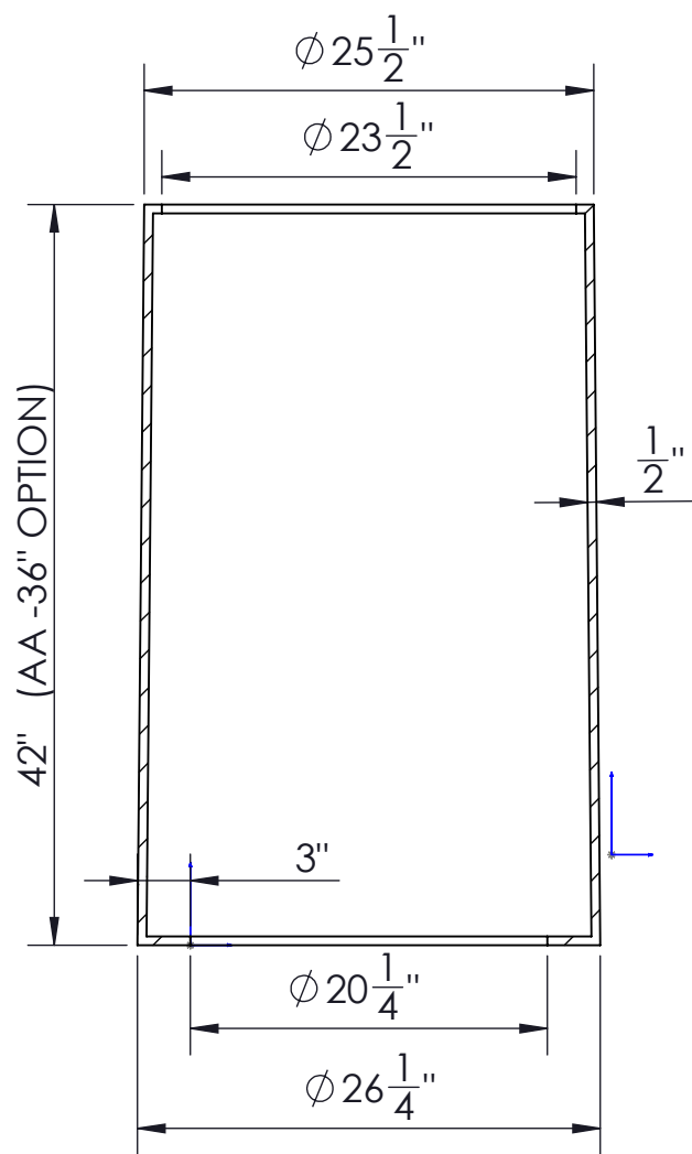
A - LD 42" HANDHOLE (2442HD5)
