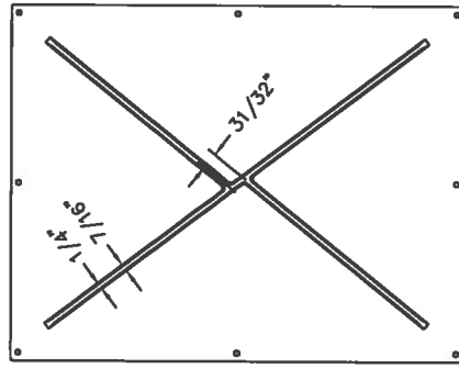
BOTTOM VIEW OF COVER
