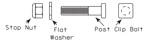
Post Clip
